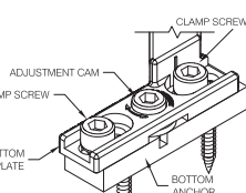
BOTTOM PIVOT ADJUSTMENT
