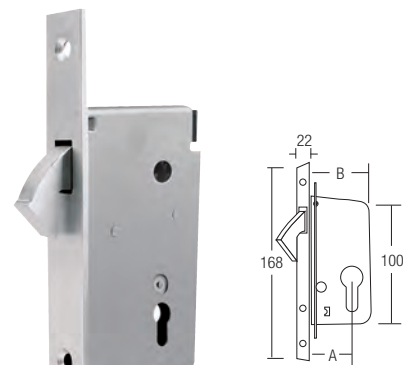
SUS304 Hook Lock
