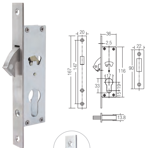
SUS304 Front Plate & Striker Plate
